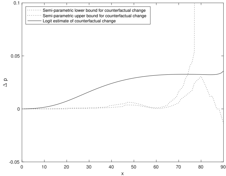
Figure 3: Counterfactual Change in Choice Probabilities using Rust Data
