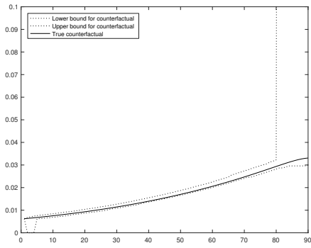
(a) \beta = .9 , using Corollary 1.
