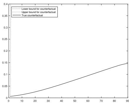
(g) \beta = .999 , using Corollary 1.
