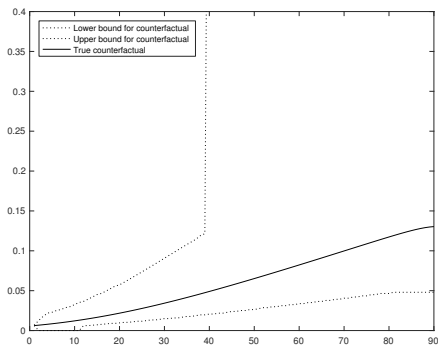
(e) \beta = .99 , using Corollary 1.
