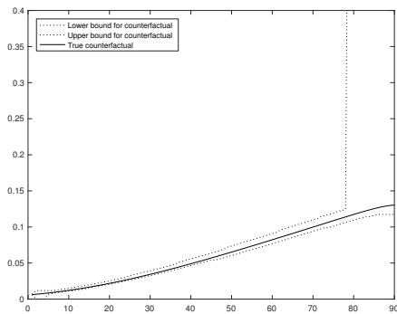
(f) \beta = .99 , using Corollaries 3 and 4.
