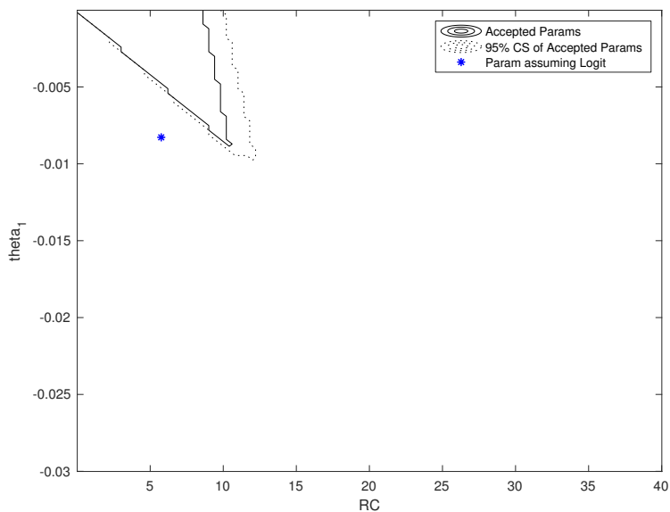
Figure 2: Accepted parameters using the Rust data
