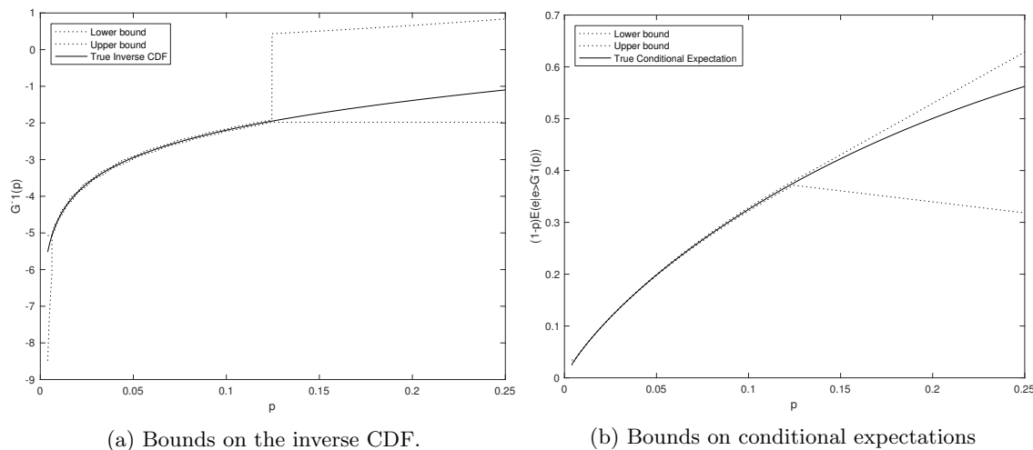
Figure 4: Bounds on the distribution of the error term based on Lemma 3 using simulated data, given true flow payoffs \pi .
