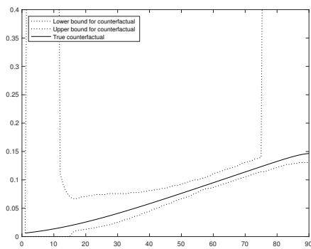
(h) \beta = .999 , using Corollaries 3 and 4.
