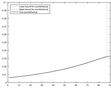
(b) \beta = .9 , using Corollaries 3 and 4.
