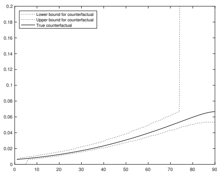
(c) \beta = .95 , using Corollary 1.
