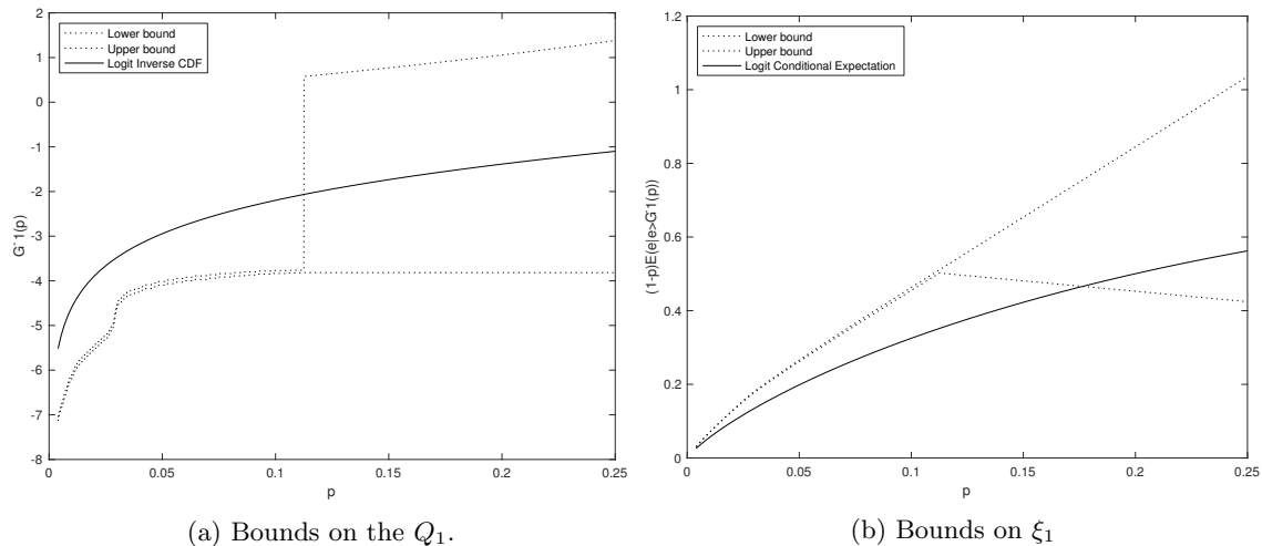
Figure 1: Bounds on the distribution of the error term based on Lemma 3 with Rust (1987) data, given a random set of accepted flow payoffs \pi .
